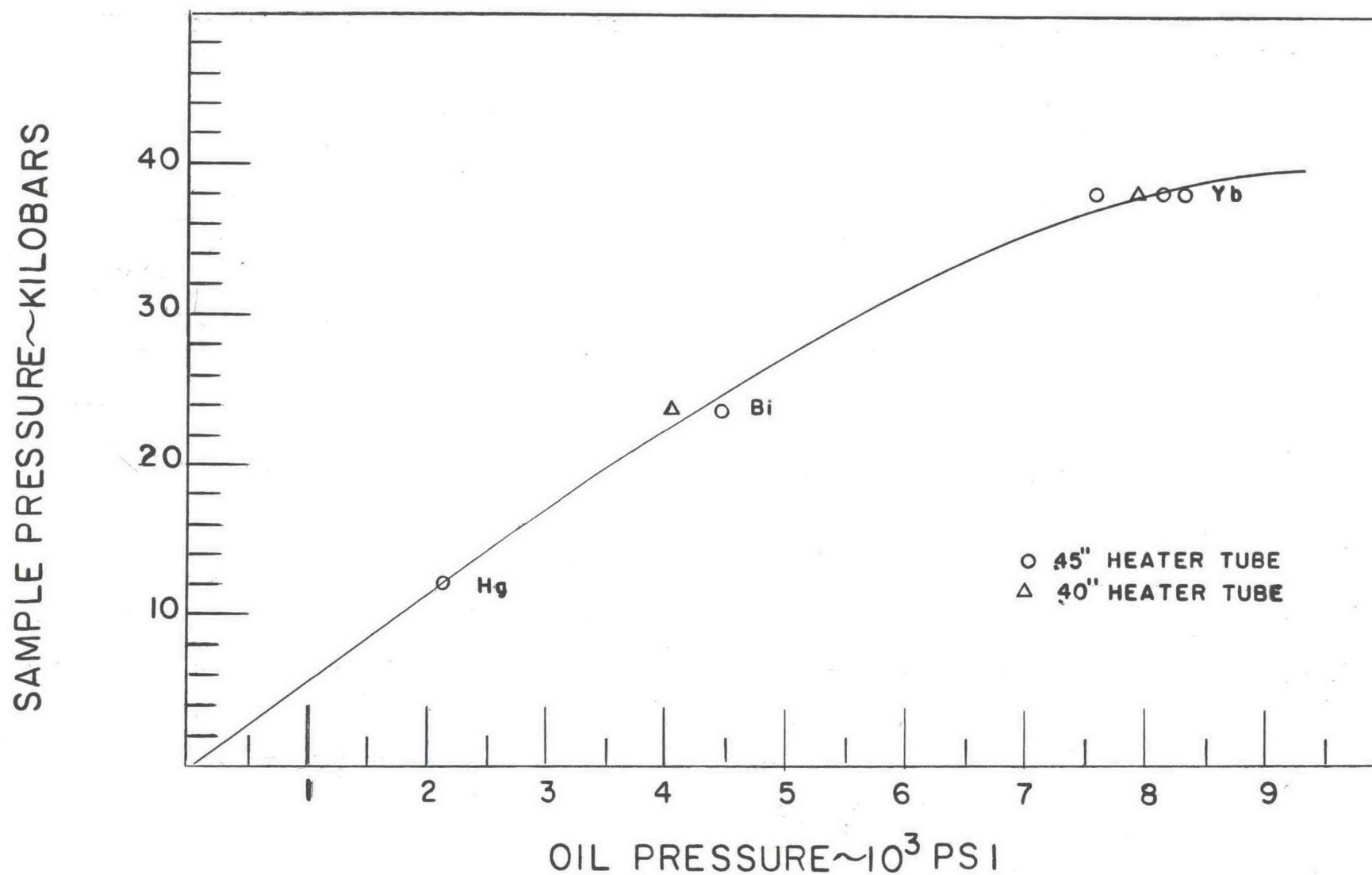
Figure 13. Calibration Curve for The Sample Geometry of This Investigation, Using The NaCl Pressure Scale
